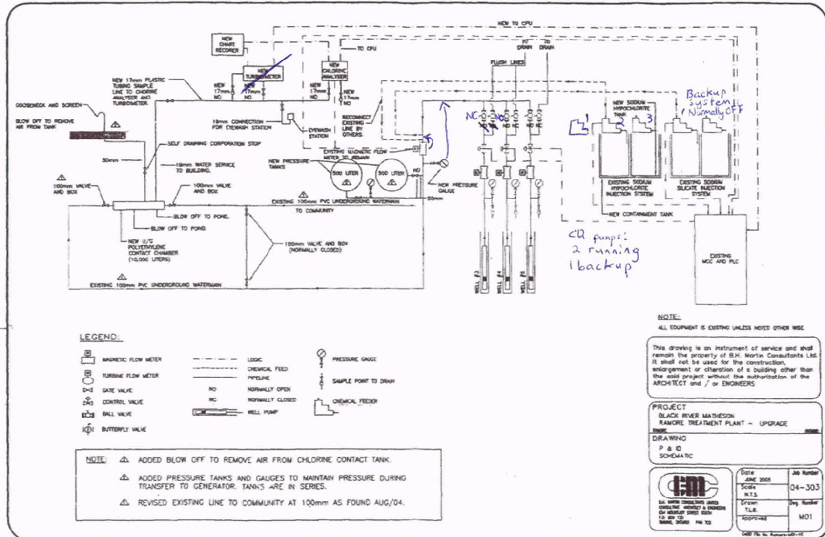
Figure 1 – Ramore Process Flow Chart
